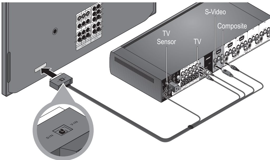
Figure 12 SCART composite video connections
